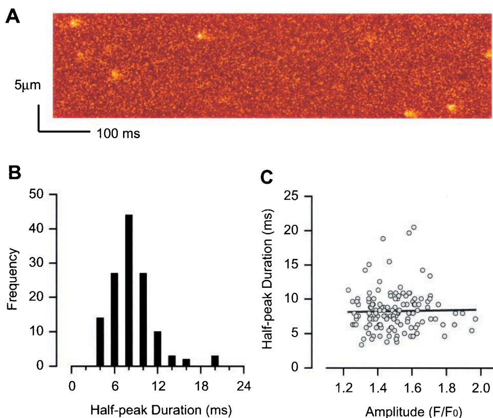
FIGURE 1 Duration of spontaneous \text{Ca}^{2+} spikes recorded with the fast \text{Ca}^{2+} indicator OG-5N (1 mM) combined with EGTA (4 mM) in cardiac myocytes. (A) A confocal image of representative \text{Ca}^{2+} spikes at a holding potential of -60 mV. The time courses of \text{Ca}^{2+} spikes (traces beneath the image) provide a measure of \text{Ca}^{2+} release function during \text{Ca}^{2+} sparks. (B) Histogram distributions for spike half-peak duration. Note that \text{Ca}^{2+} release duration for the randomly sampled population of \text{Ca}^{2+} spikes exhibits a prominent mode, in contrast to what is predicted from reversible channel gating. (C) Scatter plot of spike duration as a function of spike amplitude. Linear regression of the data (straight line) reveals no significant correlation between amplitude and duration of \text{Ca}^{2+} spikes.
