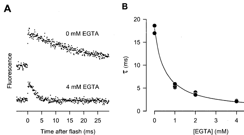
FIGURE 2 Kinetic calibration of the OG-5N/EGTA system. (A) Representative OG-5N fluorescence traces obtained with 0 and 4 mM EGTA. Note that the peak, the decaying kinetics, and the steady-state OG-5N signal after flash depend on [EGTA] used. Calibration solution was composed of (in mM) 140 KCl, 10 NaCl, 10 HEPES, 0.2 NP-EGTA, 0.15 CaCl 2 , 1 OG-5N, and 0–4 EGTA. A Ca 2+ pulse was elicited by uncaging Ca 2+ from NP-EGTA-Ca 2+ with a single 6-ns UV laser flash. (B) Relationship between the decay time constant ( \tau ) and [EGTA]. Data were fitted to a hyperbolic function, \tau = 8.99/([EGTA] + 0.505) (solid line).
