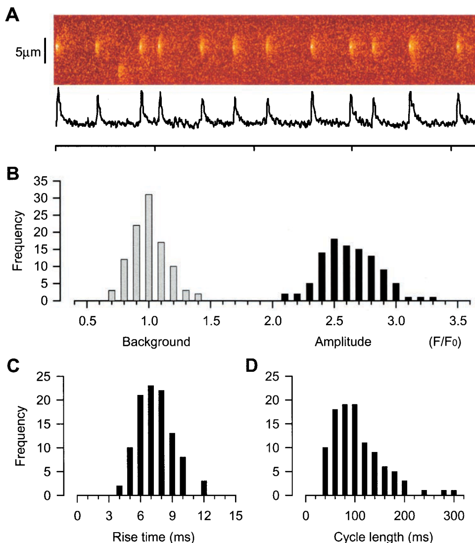
FIGURE 3 Amplitude, rise time, and cycle length of spontaneous \text{Ca}^{2+} sparks at a fixed site. (A) A typical confocal line scan image record. A total of 104 events from the hyperactive site were registered in 11 consecutive images taken over a period of 9 min in a rat cardiac myocyte at a holding potential of -60 mV. (B) Histogram distributions of spark amplitude (solid bars) and randomly sampled baseline (open bars). (C and D) Histograms for spark rise time (C) and cycle length (D).
