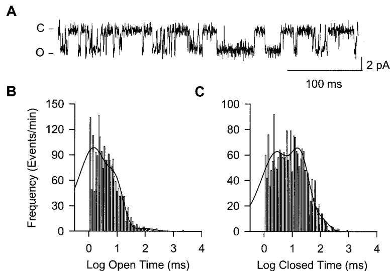
FIGURE 4 Single channel current and maximum likelihood fits of time histograms. (A) A single cardiac RyR ion channel was incorporated in a lipid bilayer. Single channel currents were recorded at 0 mV (downward deflection from closed level (c-) in symmetric 0.25 M KCl, pH 7.4 solutions containing 10 mM luminal Ca 2+ and 4 \mu M cytosolic Ca 2+ . (B and C) Open (B) and closed (C) time histograms were well-fitted by three (open time) or three (closed time) exponential functions (solid lines) with (B) a_1 = 0.476 , a_2 = 0.502 , a_3 = 0.022 , \tau_1 = 1.0 , \tau_2 = 6.2 , \tau_3 = 92.7 ms; and (C) a_1 = 0.359 , a_2 = 0.529 , a_3 = 0.113 , \tau_1 = 1.7 , \tau_2 = 14.2 , and \tau_3 = 66.5 ms (C), respectively.
