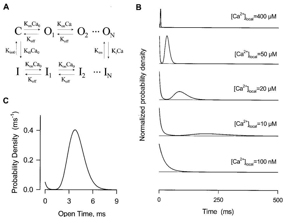
FIGURE 5 [Ca^{2+}] as a timing mechanism of RyR open time duration. (A) A contrived RyR model, where K_{on} = 10 \text{ ms}^{-1} \text{ mM}^{-1} ; K_{off} = 0.04 \text{ ms}^{-1} ; K_i = 12.8 \text{ ms}^{-1} \text{ mM}^{-1} ; K_{im} = 0.000078125 \text{ ms}^{-1} ; K_{im0} = K_{im} ; Ca_0 = 0.0001 \text{ mM} (ambient [Ca^{2+}] with the channel closed); Ca = \text{local } [Ca^{2+}] when the channel is open; and K_{io} is determined by microscopic reversibility under equilibrium conditions ( Ca = Ca_0 ). (B) Channel open duration at various local [Ca^{2+}] ranging from 100 nM to 400 \mu\text{M} . Note that the shape of distribution curve is no longer monotonically decreasing at local [Ca^{2+}] higher than 100 nM, violating the microscopic reversibility. Note also that the increase in local [Ca^{2+}] initially prolongs, but then abbreviates, the channel mean open time. This reproduces a recent experimental finding on a biphasic dependence of RyR open duration on local [Ca^{2+}] (Xu and Meissner, 1998). Interestingly, the abbreviation of channel open time at high local [Ca^{2+}] is due not only to a Ca^{2+} -dependent inactivation ( O_N \rightarrow I_N in A), but more importantly, to a Ca^{2+} -driven rapid passage through the open states ( O_1 \rightarrow O_2 \rightarrow \dots \rightarrow O_N ). (C) Open time distribution at 400 \mu\text{M} local [Ca^{2+}] on an expanded time scale. Because the local [Ca^{2+}] is much greater than the ambient [Ca^{2+}] , the clockwise reaction predominates the counterclockwise reaction, and the local high [Ca^{2+}] propels the channel through multiple consecutive open states, giving rise to a preferred open duration.
