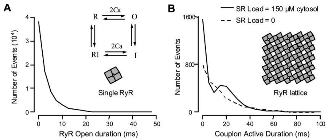
FIGURE 6 A couplon model: local CICR as a timing mechanism. A stochastic local-control model of cardiac excitation-contraction coupling was generated as in Stern et al. (1999). (A) RyR gating scheme used ( inset ) and the corresponding open time distribution. (B) Distribution of duration of couplon activation (presence of one or more open RyRs in a diad junctional complex containing a 5 \times 5 array of RyRs). The inset shows disposition of RyRs in the release unit. Their gating scheme is the same as in A. See Stern et al. (1999) for intra-couplon Ca 2+ gradients that drive irreversible gating of the unit. The distribution has a clear modal component due to the local recruitment of RyRs by CICR driven by permeating Ca 2+ . As expected, the mode disappears when the SR luminal [Ca 2+ ] is set to zero.
